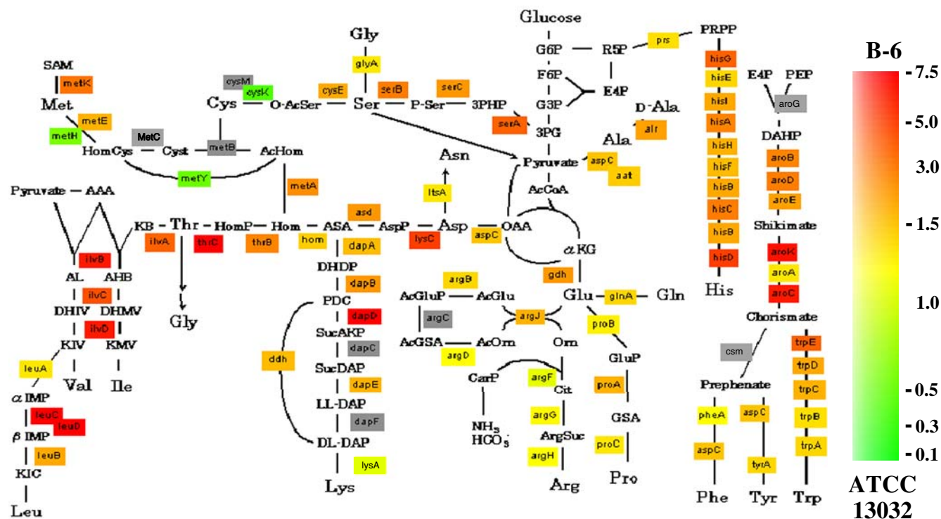
Fig. 5 mRNA levels of amino acid-biosynthetic pathway genes in industrial strain B-6 relative to those in wild-type ATCC 13032. Reddish boxes represent genes the expression of which was increased, and green boxes represent genes the expression of which was decreased in strain B-6. Genes with the P values > 0.001 are
