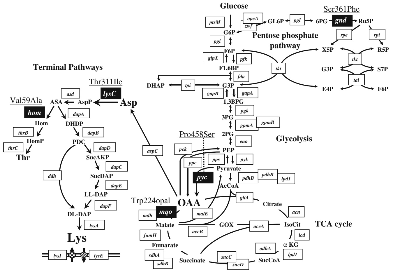
Fig. 2 L-Lysine-biosynthetic pathways and the relevant genes in C. glutamicum . The five positive mutations identified are indicated above the corresponding gene symbols
