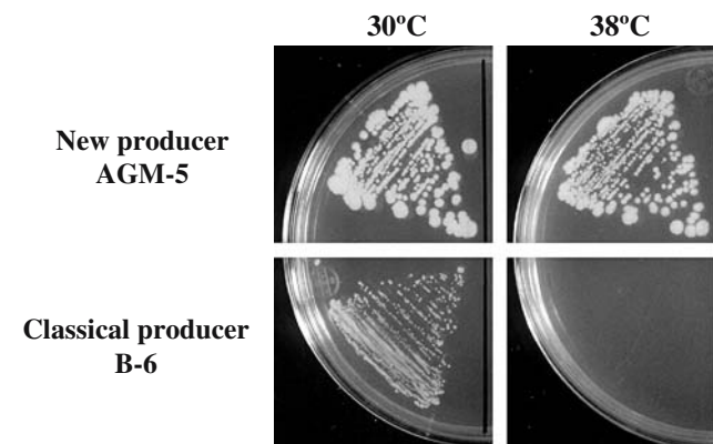
Fig. 4 Comparison of growth of the minimally mutated strain AGM-5 and the classically derived industrial producer B-6 at 30°C and 38°C. Both strains were streaked on MM plates, followed by incubation for 2 days at the temperatures indicated. The classical strain B-6 showed no growth at 38°C
